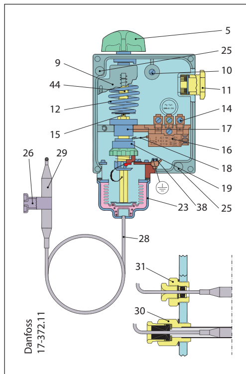
RT thermostat
